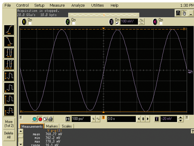
Figure 5. V p-p measurement on Agilent scope
