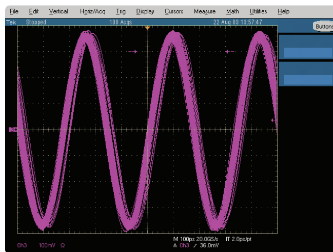
Figure 8. Visual distortion test using infinite persistence on the Tektronix scope
