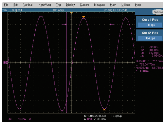
Figure 6. V p-p measurement on Tektronix scope
