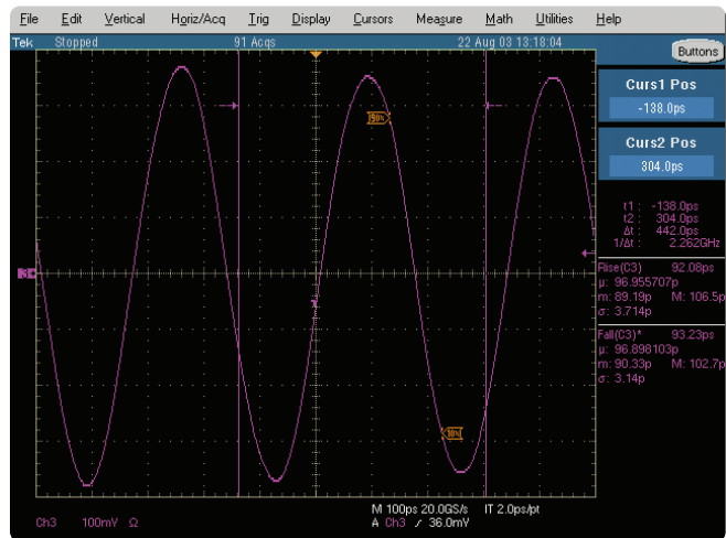
Figure 4. Rise/fall times on the Tektronix scope
