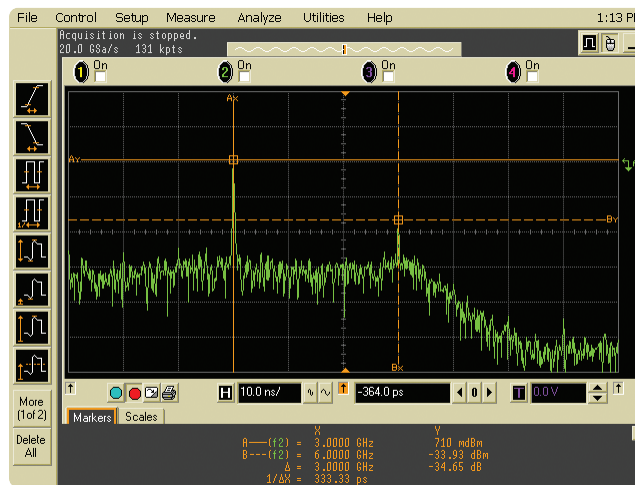
Figure 1. FFT analysis on Agilent oscilloscope
