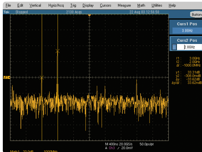
Figure 2. FFT analysis on Tektronix oscilloscope
